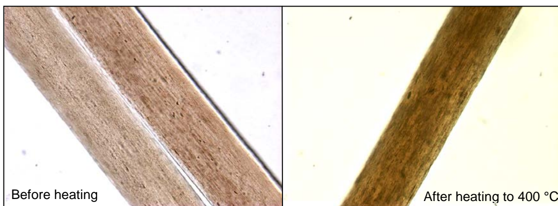
Figure 6: Two photomicrographs of a hair from Study 1. The image on the left depicts two hairs (side by side) prior to heat exposure. The image on the right depicts a hair that was exposed to a temperature of 400 °C. It shows a slight color change but bubbling and expansion are not observed. Both photos were originally taken at 400x magnification.
