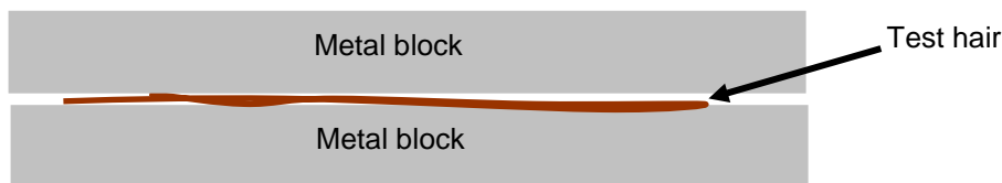
Figure 1: A diagram of the test apparatus inserted into the furnace in Study 1. The hairs were pressed between the metal blocks that are shown partially inserted into the open furnace.
